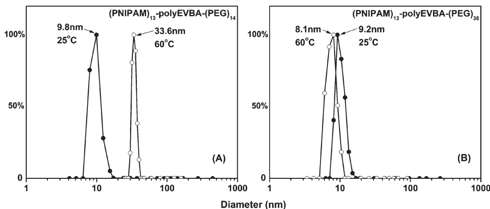
Figure 5. Size distributions (measure by dynamic light scattering at scattering angle 90^\circ ) of the (\text{PNIPAM})_{13}\text{-polyEVBA-(PEG)}_m miktoarm star copolymers at 25 and 60^\circ\text{C} . (A) m = 14 ; (B) m = 38 .
